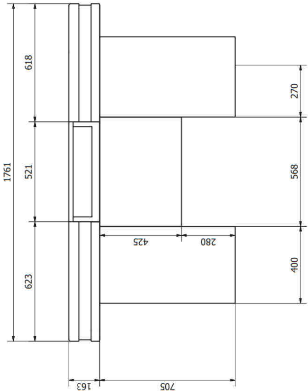
FRONT ELEVATION ( 1 : 10 )
