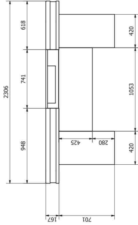
FRONT ELEVATION ( 1 : 15 )
