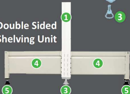
Gondola Shelving Unit Side View
